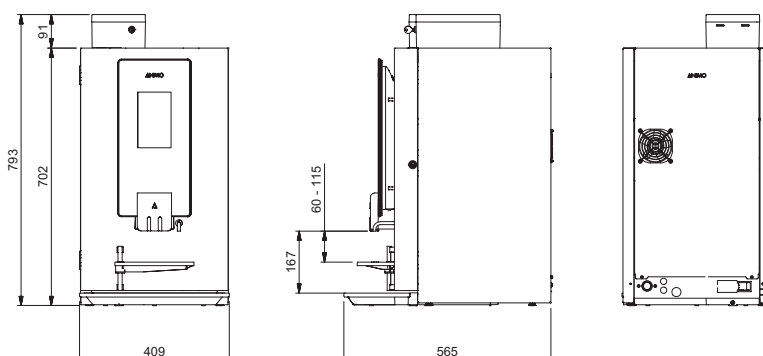
FRONT VIEW All dimensions in millimeters.
